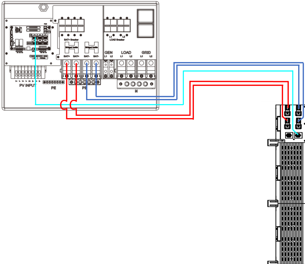
Figure 13: ETHOS with EG4 18 KPV Hybrid Inverter Connections
