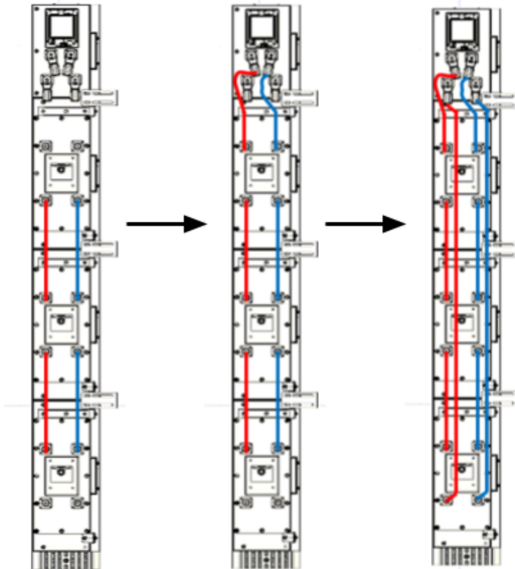
Figure 10: Parallel battery connection diagram
