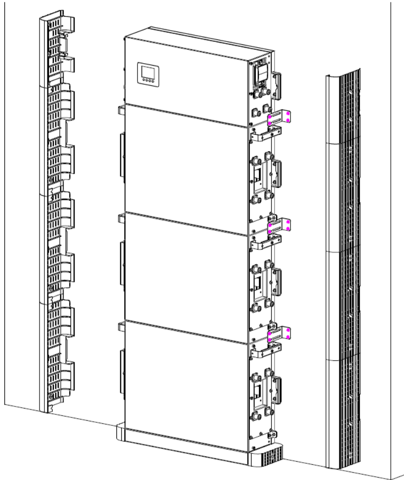
Figure 11: Side panel installation
