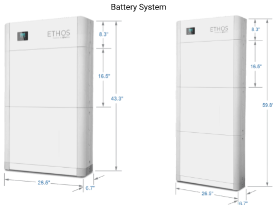
Figure 2: ETHOS System Overview
