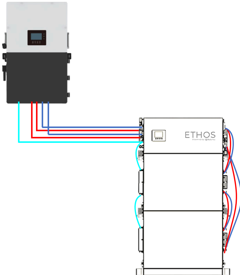
Figure 12: ETHOS with EG4 18 KPV Hybrid Inverter
