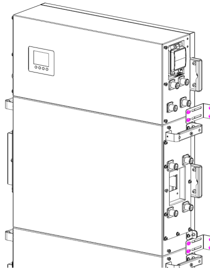
Figure 8: L bracket installation
