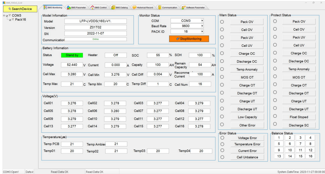
Figure 22: BMS Tools connected screen
