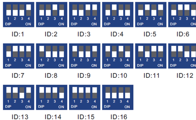
Figure 5: ETHOS Battery ID Description
