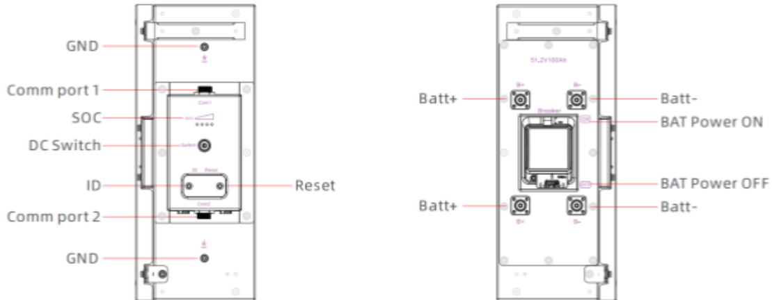
Figure 3: ETHOS Battery Diagram
