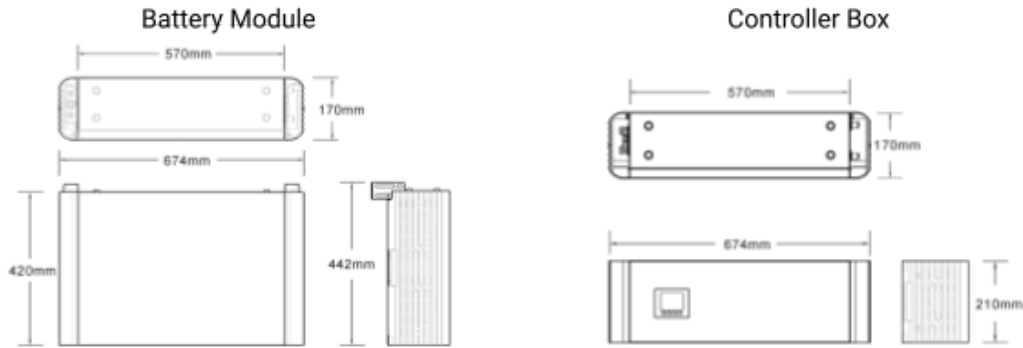
Figure 1: ETHOS Battery and Control Box Overview
