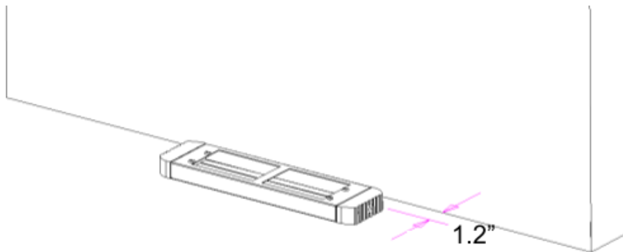
Figure 5: Bottom base installation
